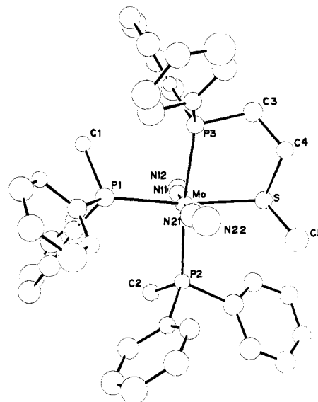
Figure 1. Molecular structure of I.
